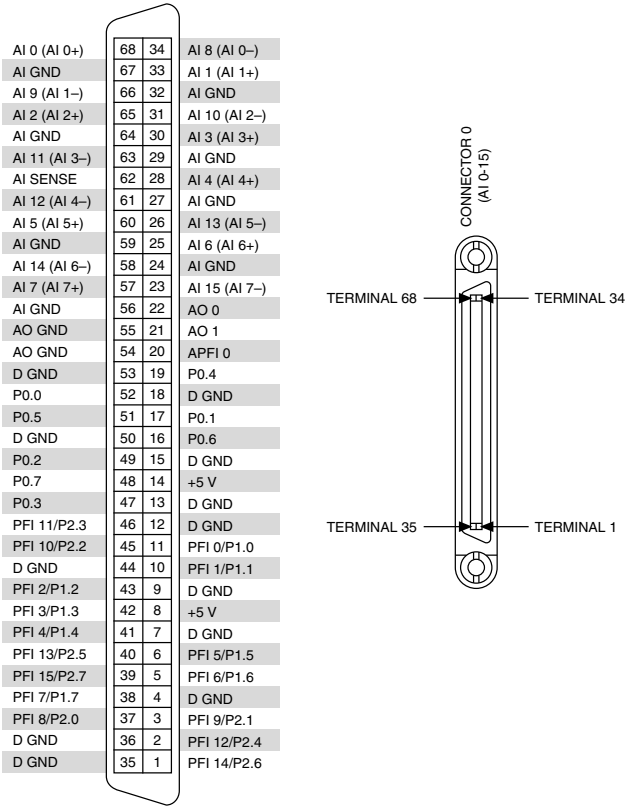
Figure 9. NI PCIe/PXIe-6361 Pinout
